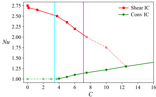
Figure 18. Nusselt number versus C for simulations started with shear and convection initial conditions (ICs) at Re = 5300 . The magenta and cyan vertical lines correspond to the critical buoyancy parameters C_{cr,1} and C_{cr,2} given by (3.12) and (3.15), respectively. For values of C \gtrsim C_{cr,1} ( C \lesssim C_{cr,2} ) the shear-driven (convection-driven) state is not supported and correspondingly the upper (lower) branch is plotted with a dashed semitransparent line.
