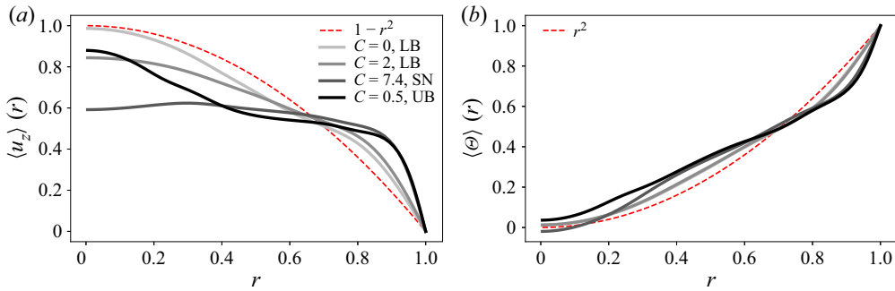
Figure 11. Mean streamwise velocity (a) and temperature (b) profiles at the points along the continuation from N4L ( Re = 2500 ) marked in figure 10 (SN: saddle node, LB/UB: lower/upper branch). The temperature profiles for C = 0 and C = 2 on the lower branch are indistinguishable.
