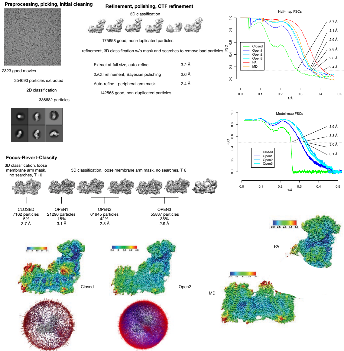
Fig. S5. Processing of the rotenone cryo-EM dataset.
