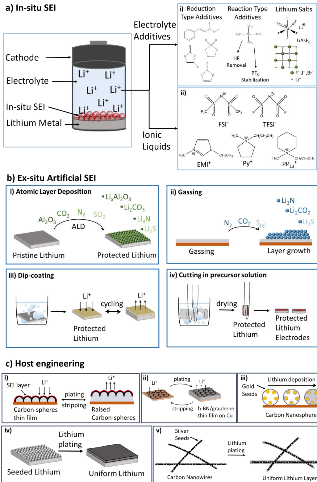
Figure 2. Overview of the main stabilization methods for lithium metal anodes in liquid electrolyte. a) “in-situ” SEI, b) “ex-situ” artificial SEI and c) host structures. a) “in-situ” SEIs can be tailored via i) electrolyte additives or ii) ionic liquids. b) “ex-situ” artificial SEIs can be produced by i) atomic layer deposition, ii) gassing, iii) dip-coating or iv) cutting of lithium in a precursor solution. c) stabilizing host structures can consist of i) a carbon-sphere thin film, ii) a h-BN/graphene thin film, iii) hollow carbon nanospheres, iv) a ultrafine lithium seed layer or v) seeded carbon nanowires.
