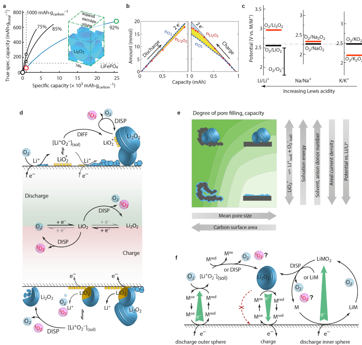
Figure 7: a , True capacity of a Li-O 2 cathode as a function of capacity per mass of carbon for three cases of initial porosity (given by percentages above the curves), which is filled to 80%. The black squares and red circles at 1,000 \text{mAh}\cdot\text{g}_{\text{carbon}}^{-1} illustrate that respective true capacities vary strongly with electrode architecture. Value for the intercalation material \text{LiFePO}_4 is given by the dashed line for comparison. The insert shows the space filling of spherical \text{Li}_2\text{O}_2 particles inside the porous electrode and the displaced electrolyte volume at 25,000 \text{mAh}\cdot\text{g}_{\text{carbon}}^{-1} for 92% initial porosity (indicated by the green circle). Adapted with permission from Ref.[305], NPG. b , Typical moles of \text{O}_2 and \text{Li}_2\text{O}_2 involved upon discharge and charge. Adapted with permission from Ref.[307], NPG. c , Thermodynamics of alkali peroxides and superoxides. Standard potentials of the \text{O}_2/\text{MO}_2 and \text{O}_2/\text{M}_2\text{O}_2 redox couples on the \text{M}/\text{M}^+ scales with \text{M} = \text{Li}, \text{Na}, \text{K} . The scales are brought to a common scale based on their \text{M}/\text{M}^+ standard potentials. The dashed horizontal line indicates the \text{O}_2/\text{KO}_2 couple. The \text{O}_2/\text{LiO}_2 potential is adopted from Ref.[308]. With permission from Ref.[309], Royal Society of Chemistry. d , Overview of the discharge and charge process with dominant disproportionation steps for the 2 nd e^- transfer and concurrent {}^3\text{O}_2/{}^1\text{O}_2 release (centre). From Ref.[309], Royal Society of Chemistry. Steps are more detailed for discharge/charge on top/bottom. e , Parameters determining product morphology and degree of pore filling. f , Processes upon mediated discharge and charge and open questions regarding {}^1\text{O}_2 formation.
