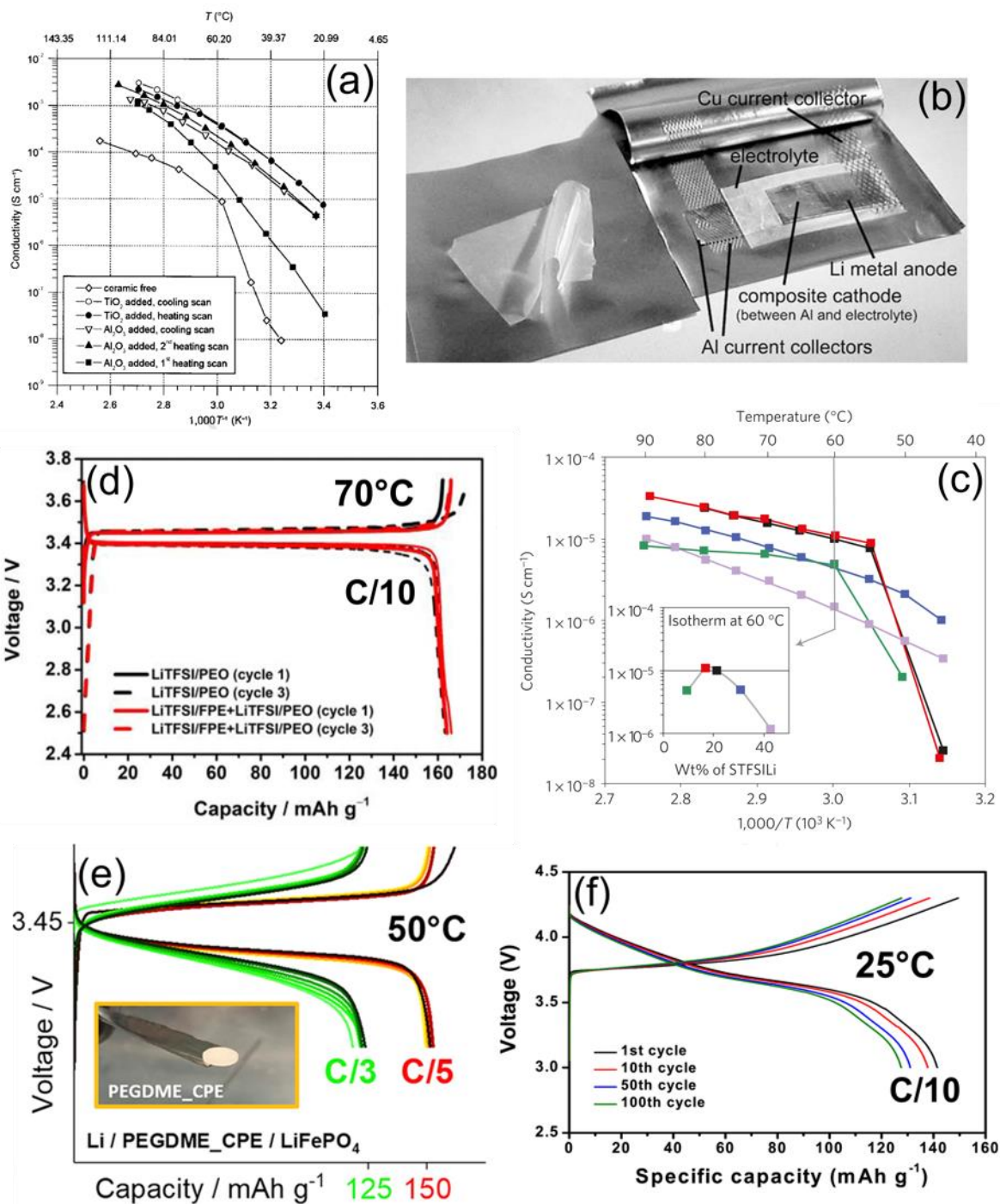
Figure 4 - (a) Temperature dependence of the ionic conductivity of various nano-sized oxide-PEO composite polymer electrolytes [189]; (b) free-standing PEO-LiTFSI membrane containing 150 wt.% PYR 13 TFSI and solid-state LMP battery consisting of a Cu current collector, Li metal anode, SPE, composite cathode and Al current collectors [196]; (c) temperature dependence of the ionic conductivity for several single-ion block copolymer electrolytes comprising polystyrene segments [ i.e. , poly(styrene trifluoromethanesulphonylimide of lithium), P(STFSILi)], with (inset) isothermal conductivity at 60^{\circ}\text{C} according to the wt% of the P(STFSILi) block [197]; (d) voltage profiles of a Li|LiTFSI-PEO|LFP cell using an amorphous polymeric interlayer at the anode side at 70^{\circ}\text{C} under a constant current of C/10 [198]; (e) voltage profiles of a Li|PEGDME|LFP cell [where PEGDME is poly(ethylene glycol) dimethyl ether] at 50^{\circ}\text{C} under constant current rates of C/5
