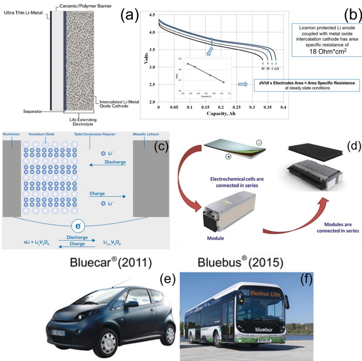
Figure 5: (a) schematic of a Licerion ® cell employing an ionically conductive ceramic/polymer barrier protecting the lithium electrode and a high-voltage metal-oxide intercalation cathode, (b) corresponding discharge voltage profile at various current rates ranging from C/3 to 3C and voltage vs. current at steady-state conditions [216]; (c) schematic of the lithium-metal battery prototype developed in the 1990s, comprising a Li anode, a PEO-LiClO 4 /LiTFSI electrolyte, and a VO x cathode [217]; (d) schematic of assembly of a LMP ® battery pack (developed and commercialized by the Bolloré Group) from the cell level [204]; (e) Bluecar and (f) Bluebus (using the LMP ® technology) commercialized by the Bolloré Group [218].
