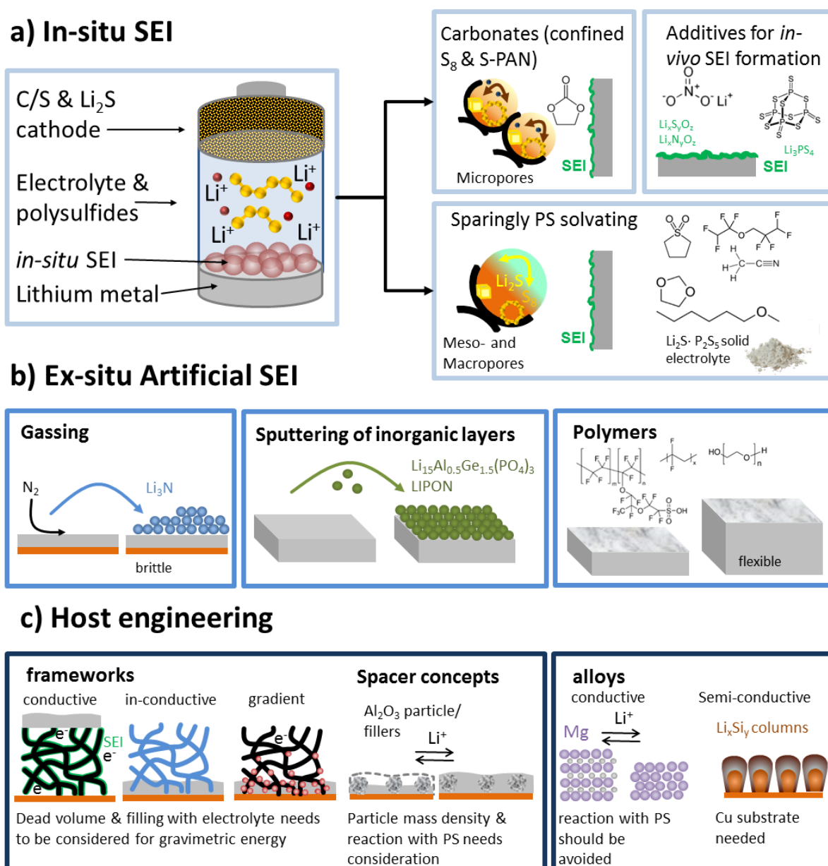
Figure 6. Overview of the main stabilization methods for lithium metal anodes in liquid electrolyte being adapted for Li-S batteries. a) "in-situ" SEI with carbonates for confined sulfur species in the cathode pores, additives for in-vivo SEI formation and sparingly polysulfide solvating electrolytes as approach to intrinsically hinder anode corrosion by polysulfides. b) "ex-situ" artificial SEI by gassing, sputtering of inorganic layers, and application of polymers. c) host engineering by conductive and inconductive frameworks, spacer concepts, and alloys.
