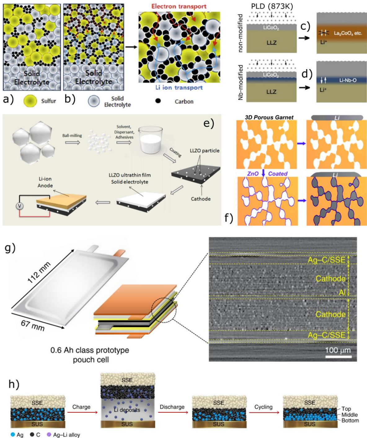
Figure 3. Optimization of the cathode- and anode-electrolyte interfaces in ASSBs. Schematics of lithium ion and electron transport in a sulphur-based composite cathode consisting of large particles with (a) non-homogeneous distribution and (b) small particles with homogeneous distribution. Reprinted with permission from [144]. © 2017 Elsevier. Schematic illustrations of (c) non-modified and (d) Nb-modified LLZO/LiCoO 2 interfaces. The mutual diffusion between LLZO and LiCoO 2 produces non-Li + -conductive phases such as La 2 CoO 4 . The Nb-modified surface suppresses the mutual diffusion and produce Li + -conductive amorphous phase. Reprinted with permission from [140]. © 2014 Elsevier. (e) Schematic illustration of the fabrication of an ultrathin electrolyte all-solid-state Li/LLZO/LiFePO 4 battery. Reprinted with permission from [150]. © 2017 American Chemical Society. (f) Schematic illustration of the lithium melt infusion into 3D porous garnet with or without
