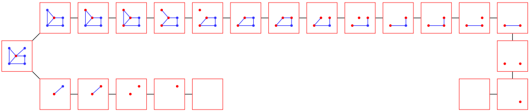
Fig. 6. A nice tree decomposition of the graph in Figure 2. The leftmost node is the root. The graph G_t is illustrated in each node t . The vertices of the bags X_t are shown in red.
