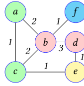
Fig. 7. An optimal 2-partitioning
