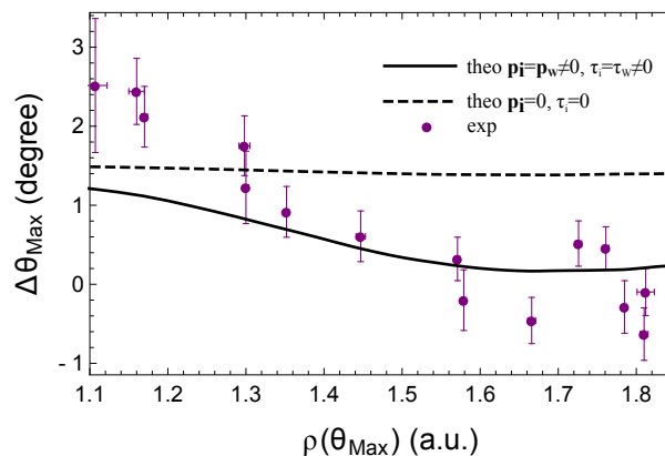
Figure 7. Difference between the most probable photoelectron emission angle for argon and krypton. Experiment and theory (with and without initial momentum and tunneling delay time). Adapted from [23].
