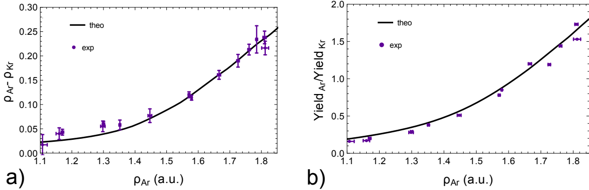
Figure 6. Comparison of the experiment and the theory; a) the difference between the average electron momentum, b) the yield ratio. Adapted from [23].
