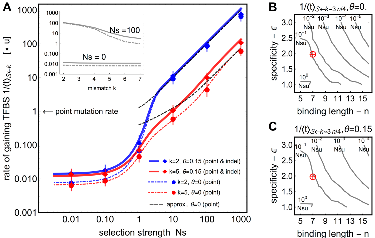
Fig 2. Single TF binding site gain rates at an isolated DNA region. A) The dependence of the gain rate, 1/\langle t \rangle_{S \leftarrow k} shown in units of point mutation rate, from sequences in different initial mismatch classes k (blue: k = 2 , red: k = 5 ), as a function of selection strength. Results with point mutations only ( \theta = 0 ) are shown by dashed line; with admixture of indel mutations ( \theta = 0.15 ) by a solid line. For strong selection, Ns \gg n \log(2)/2 , the rates scale with Ns , which is captured well by the “shortest path” approximation (black dashed lines in the main figure) of Eq (24). The biophysical parameters are: site length n = 7 bp; binding specificity \epsilon = 2 k_B T ; chemical potential \mu = 4 k_B T . Points correspond to Wright-Fisher simulations with Nu = 0.01 where error bars cover \pm 2 SEM (standard error of mean). Inset shows the behavior of the gain rates as a function of the initial mismatch class k for Ns = 0 and Ns = 100 . B, C) Gain rates from redundancy rich classes ( k \sim 3n/4 , typical of evolution from random “virgin” sequence) under strong selection, without (B) and with (C) indel mutations supplementing the point mutations. Red crosshairs denote the cases depicted in panel A. Contour lines show constant gain rates in units of Ns u as a function of biophysical parameters n and \epsilon . Wiggles in the contour lines are not a numerical artefact but a consequence of discrete mismatch classes.
