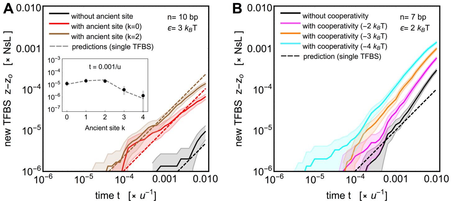
Fig 5. Ancient sites and cooperativity can accelerate the emergence of TF binding sites in longer regulatory sequences. A) The expected number of newly evolved TFBS in the presence (red and brown) or absence (black) of an ancient site, for binding site length n = 10 bp, and specificity, \epsilon = 3 k_B T . In this example, the ancient site was a consensus site ( k = 0 ) or two mismatches away from it ( k = 2 ) that evolved under neutrality for t' = 0.1/u prior to starting this simulation. Dashed lines show the predictions of a simple analytical model, Eq (30). The inset shows how the number of newly evolved TFBS at t = 0.001/u scales with the mismatch of the ancient site k (plot markers: simulation means; error bars: two standard errors of the mean; dashed curve: prediction). B) The expected number of newly evolved TFBS without (black) and with cooperative interactions (for different cooperativity strengths, magenta: E_c = -2 k_B T , yellow: E_c = -3 k_B T , cyan: E_c = -4 k_B T , see Eq (11) in Methods and text) for binding site length n = 7 bp, and specificity, \epsilon = 2 k_B T . Both panels use \mu = 4 k_B T , strong selection ( Ns = 100 ) and a combination of point and indel mutations ( \theta = 0.15 ), acting on a regulatory sequence of length L = 30 bp. Thick solid lines show an average over 1000 simulation replicates, shading denotes \pm 2 SEM.
