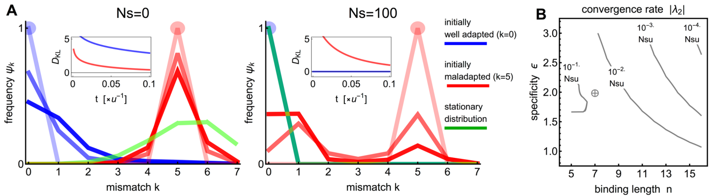
Fig 3. Convergence to the stationary distribution of TFBS sequences. A) Evolutionary dynamics of the mismatch classes distribution \psi(k) for an isolated TFBS under point and indel mutations ( \theta = 0.15 ), directional selection for stronger binding, and genetic drift is shown for initially well ( k = 0 , blue) and badly ( k = 5 , red) adapted populations. At left, no selection ( Ns = 0 ); at right, strong selection ( Ns = 100 ). Different curves show the distribution of genotype classes at different time points ( t = 0u^{-1} , 0.05u^{-1} , 0.1u^{-1} as decreasing opacity); stationary distribution is shown in green. Insets show the time evolution to convergence for initially well ( k = 0 , blue) and badly ( k = 5 , red) adapted populations, measured by the Kullback-Leibler divergence D_{KL}[\psi(t) || \psi(t = \infty)] . The biophysical parameters are: n = 7 bp, \epsilon = 2 k_B T , \mu = 4 k_B T . B) Rate of convergence to the stationary distribution for different \epsilon and n values under strong selection ( Ns \gg n \log(2)/2 ; here specifically Ns = 100 ) and for \theta = 0.15 . Crosshairs represent the parameters used in a).
