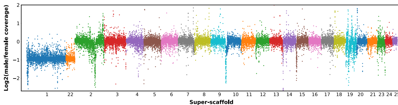
Fig. 1. Patterns of male/female coverage for the longest 25 scaffolds in 10,000 bp windows. Scaffolds 1 and 22 were classified as X-linked based on their reduced male:female coverage ratio.
