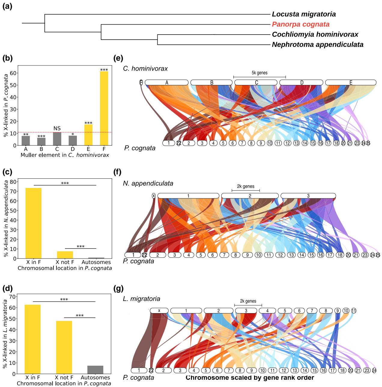
Fig. 2. Homology of the X chromosomes of P. cognata (order: Mecoptera) and 3 other insects: 2 Diptera, C. hominivorax (suborder: Brachycera) and N. appendiculata (suborder: Nematocera), and L. migratoria (order: Orthoptera). (a) Phylogenetic tree of the 4 species. (b) Percentage of genes on each of the C. hominivorax 's Muller elements that are X-linked in P. cognata . The dashed line represents the overall proportion of orthologs that are X-linked in P. cognata (i.e. the "X-linkage threshold"). (c) Percentage of X-linked and autosomal P. cognata genes that are X-linked in N. appendiculata . The X-linked genes of P. cognata were divided into 2 sets, based on whether they were F-linked in C. hominivorax (X in F), or not (X not F). (d) Same as (c) but showing the percentage of P. cognata genes that are X-linked in L. migratoria . Statistically significant differences between observed and expected percentages were assessed using a chi-squared test (* P < 0.05 , ** P < 0.01 , *** P < 0.001 , NS not significant). (e, f, g) Synteny plots between P. cognata 's 25 largest genome scaffolds and the genomes of the 3 other insect species. Note that no synteny was found between P. cognata scaffold 19 and the genomes of the other species.
