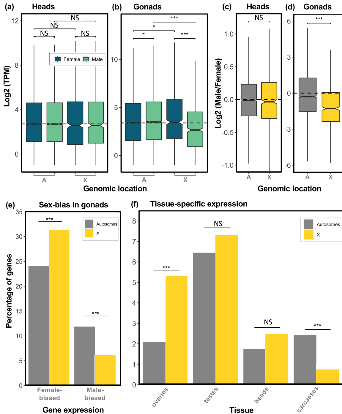
Fig. 3. Dosage compensation and biased gene content of the X. (a and b) Expression of autosomal and X-linked genes in males and females, in heads and gonads, respectively (the dashed line corresponds to the female autosomal gene expression median). (c and d) Log 2 of male-over-female expression ratios for the autosomal and X-linked genes, in heads and gonads, respectively. Statistically significant differences between groups were assessed using a Wilcoxon rank sum test (*adj. P < 0.05 , **adj. P < 0.01 , ***adj. P < 0.001 , NS not significant). (e) Percentage of autosomal and X-linked genes exhibiting sex-biased expression in gonads. (f) Percentage of autosomal and X-linked genes showing tissue-specific expression. Statistically significant differences between the autosomes and the X in (e) and (f) were assessed using a chi-squared test.
