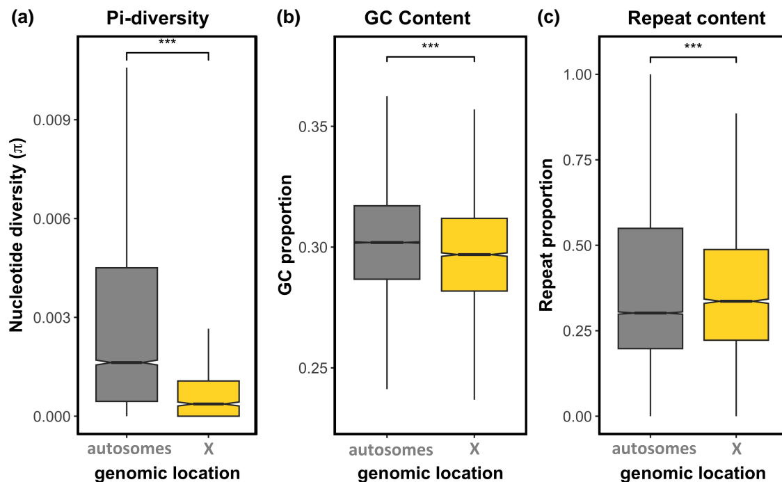
Fig. 4. X versus autosomal (a) female nucleotide diversity ( \pi ), (b) GC content, and (c) repeat content (per 10,000 bp windows). Statistically significant differences between groups were assessed using a Wilcoxon rank sum test (*adj. P < 0.05 , **adj. P < 0.01 , ***adj. P < 0.001 , NS not significant).
