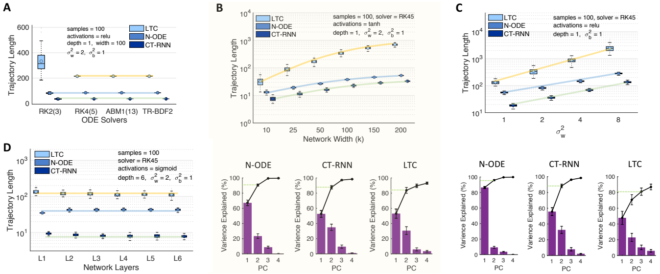
Figure 3: Dependencies of the trajectory length measure. A) trajectory length vs different solvers (variable-step solvers). RK2(3): Bogacki-Shampine Runge-Kutta (2,3) (Bogacki and Shampine 1989). RK4(5): Dormand-Prince explicit RK (4,5) (Dormand and Prince 1980). ABM1(13): Adams-Bashforth-Moulton (Shampine 1975). TR-BDF2: implicit RK solver with 1st stage trapezoidal rule and a 2nd stage backward differentiation (Hosea and Shampine 1996). B) Top: trajectory length vs network width. Bottom: Variance-explained of principle components (purple bars) and their cumulative values (solid black line). C) Trajectory length vs weights-distribution variance. D) trajectory length vs layers. (More results in the supplements)
