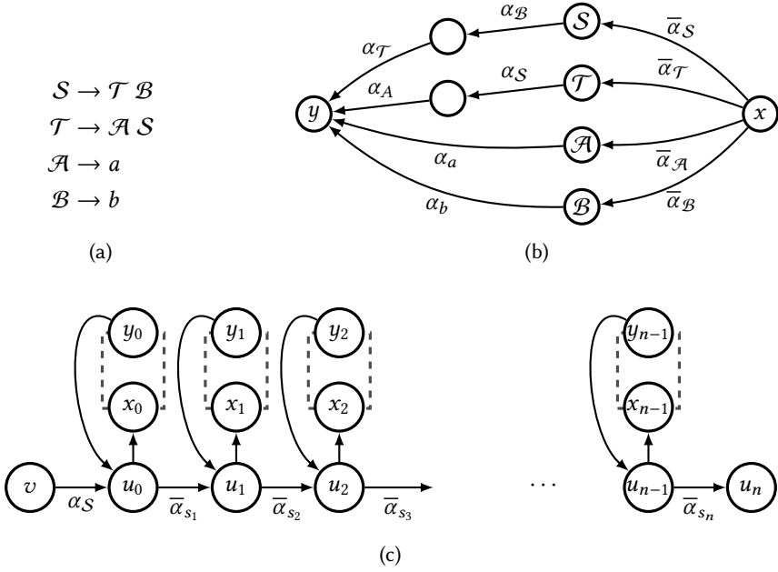
Fig. 5. (5a) A grammar \mathcal{G} for the language a^n b^n , (5b) The gadget graph G^{\mathcal{G}} , (5c) The parse graph G_s^{\mathcal{G}} , given a string s = s_1, \dots, d_n .
