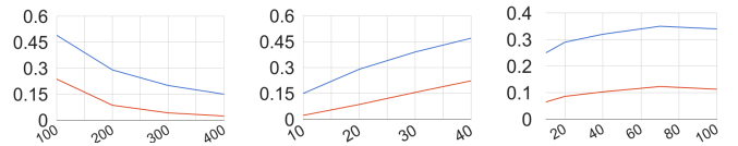
Figure 4: The ratio between the size (vertices - blue lines and edges - red lines) of the concrete and truncated networks as |V| , k , and |W| increase.
